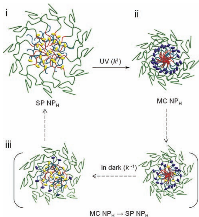
Figure 9. Proposed assembly states of reversible light-triggered SP NP H size switching: SP NP H converted MC NP H upon irradiation (solid arrow, i to ii); graduate transition (dash arrow, ii to iii to i) from MC NP H to SP NP H in the dark, with the conversion of zwitterionic MC-C9 to hydrophobic SP-C9 to cause the reassembly of NP H . Yellow oval, SP molecule; blue line, the alkyl chain in SP; red, lipid part; green line, PEG; and purple oval, MC molecule.
